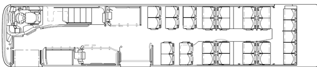
12.8m length lower deck with 31 fixed seats + 2 wheelchair spaces
