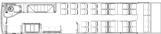
Lower deck with 33 fixed seats, 3 tip-up seats + 1 wheelchair space
