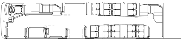
Lower deck with 18 fixed seats + 2 wheelchair spaces
