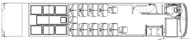
Lower deck with 21 fixed seats + 2 wheelchair positions
