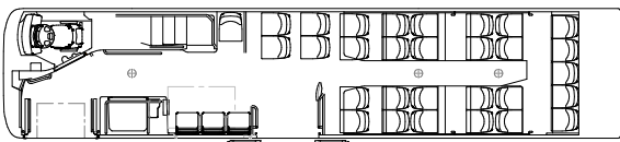
Lower deck with 30 fixed seats, 3 tip-up seats and 1 wheelchair space
