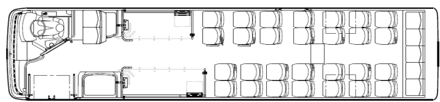
11.5m length with 35 fixed seats, 2 tip-up seats + 2 wheelchair spaces
