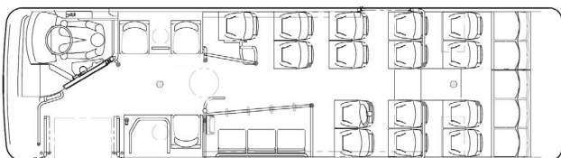
23 fixed seats, 3 tip-up seats + 1 wheelchair space
