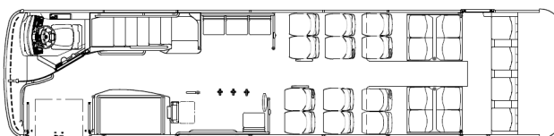
10.9m length lower deck with 24 fixed seats, 4 tip-up seats and 1 wheelchair space
