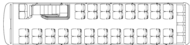
10.9m length upper deck with 46 seats
