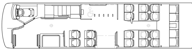
Lower deck with 20 fixed seats + 1 wheelchair space
