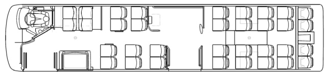
11.7m length with 34 fixed seats + 1 wheelchair space
