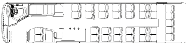
Lower deck with 33 fixed seats, 1 tip-up seat + 1 wheelchair space
